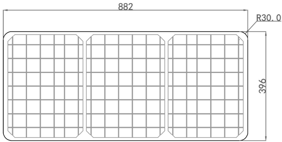
PV panel size T4.0
